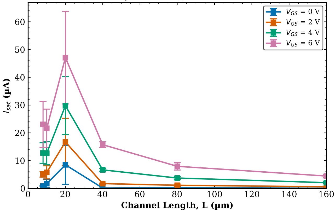
All Chips - Combined I_{sat} vs L | W = 50 \mu\text{m} (mean \pm std)
